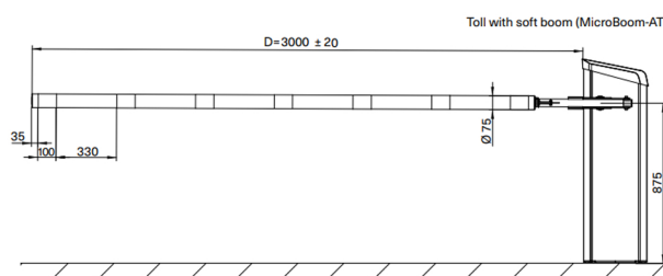
Toll with soft boom (MicroBoom-AT)
