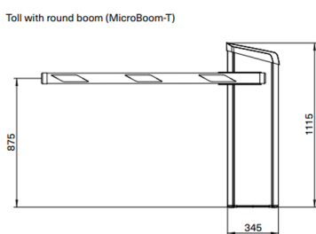
Toll with round boom (MicroBoom-T)
